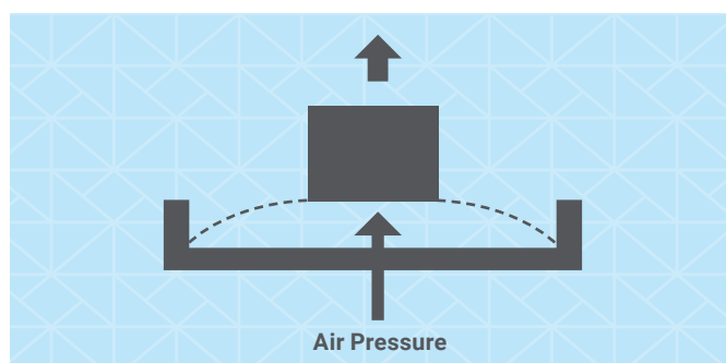
Origin's pneumatic separation mechanism applies much less separation force: the membrane gradually peels off each cured layer as the build platform goes up.
